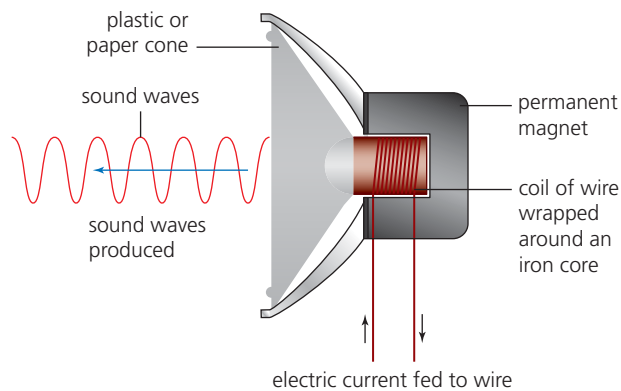
▲ Figure 3.14 Diagram showing how a loudspeaker works
