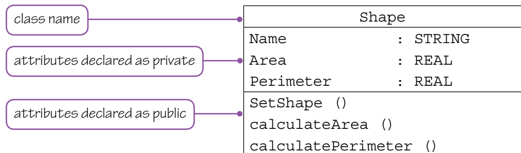
▲ Figure 20.1 Shape class diagram
