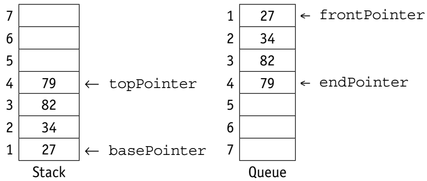
▲ Figure 10.11 Stack and queue
