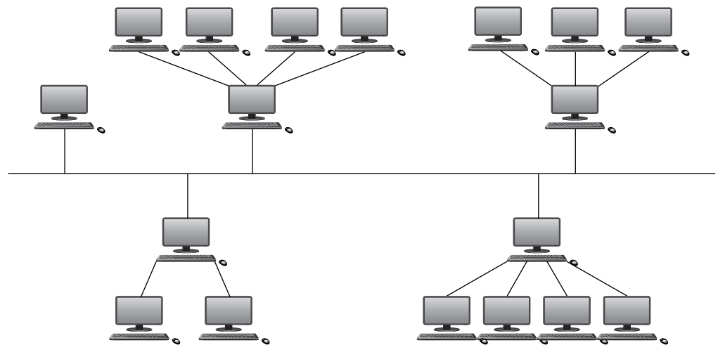
▲ Figure 2.9 Hybrid bus and star network
