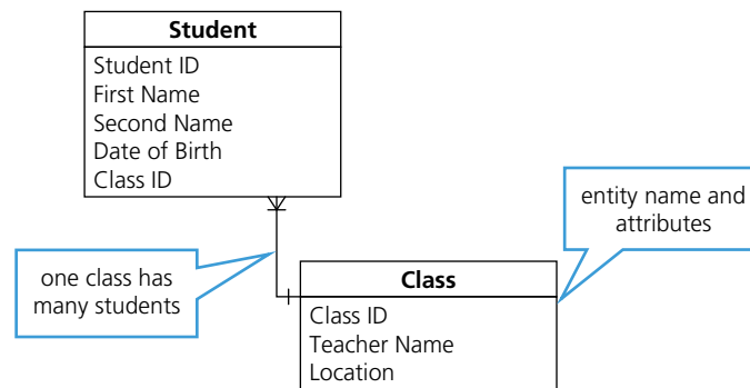
▲ Figure 8.3 E-R diagram for school database
