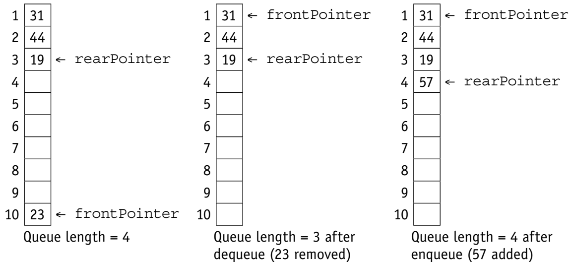
▲ Figure 10.15 Circular queue operation
