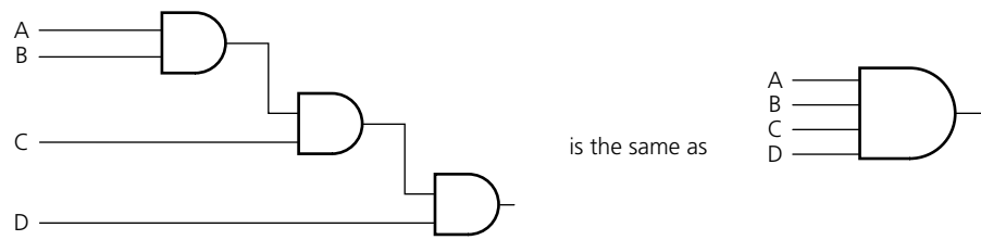
▲ Figure 3.33 4-input AND gate
