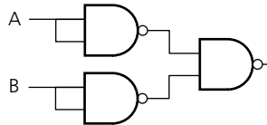
▲ Figure 3.30 OR gate made from NAND gates
