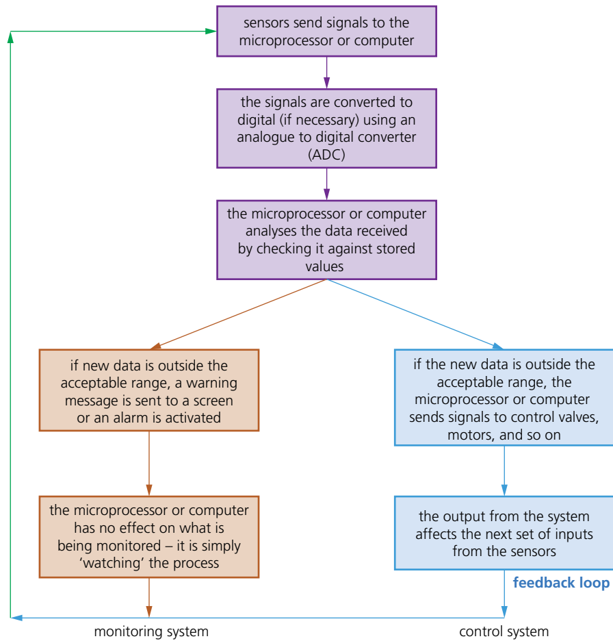
▲ Figure 3.20 Sensors for monitoring and controlling systems
