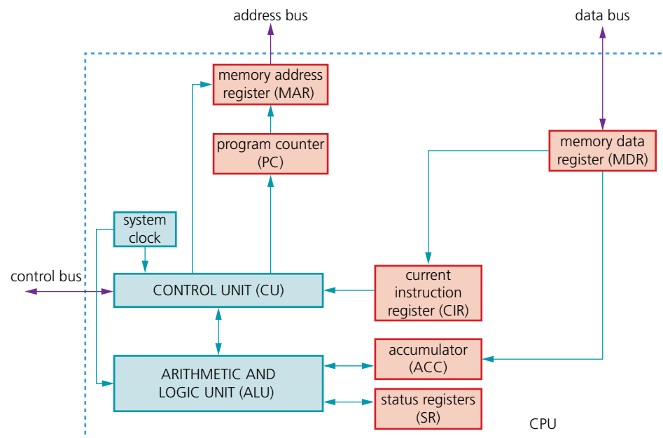
▲ Figure 4.1 Representation of Von Neumann architecture
