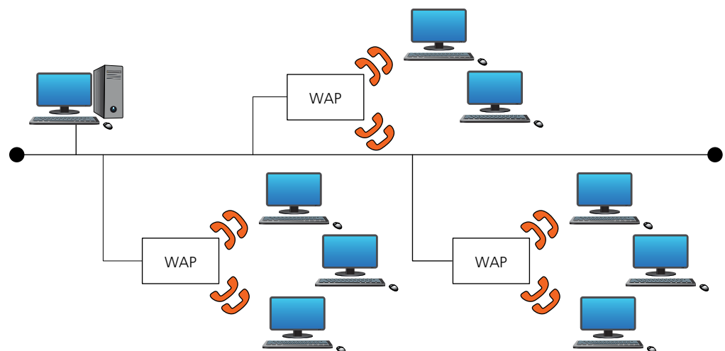
▲ Figure 2.2 Wireless local area networks (WLAN)
