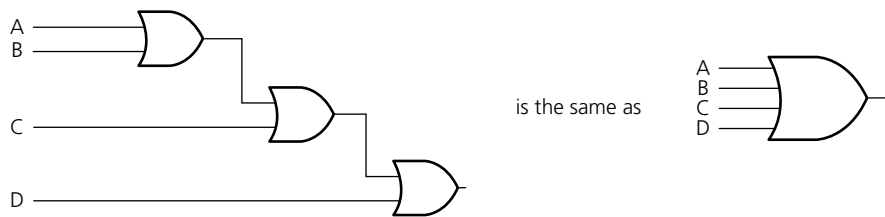
▲ Figure 3.35 4-input OR gate
