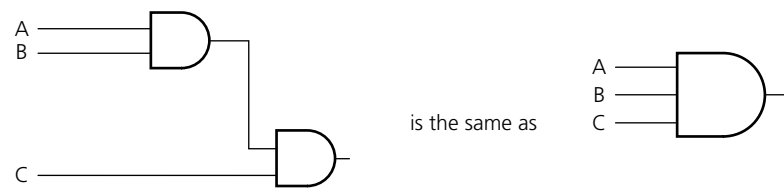
▲ Figure 3.32 Multi-input AND gate
