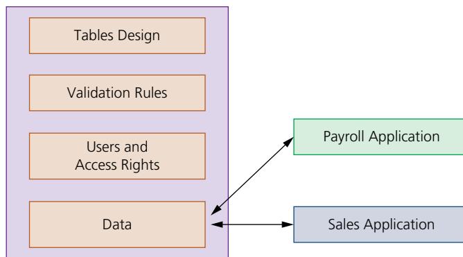
▲ Figure 8.2 Database approach
