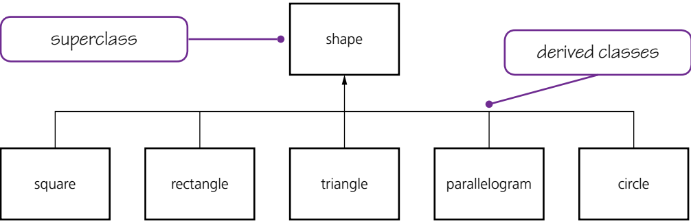
▲ Figure 20.2 Inheritance diagram – single inheritance
