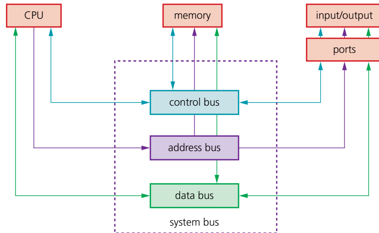
▲ Figure 4.2 System buses
