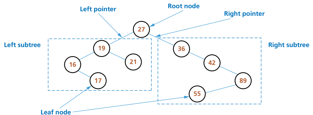
▲ Figure 19.10 Example of an ordered binary tree
