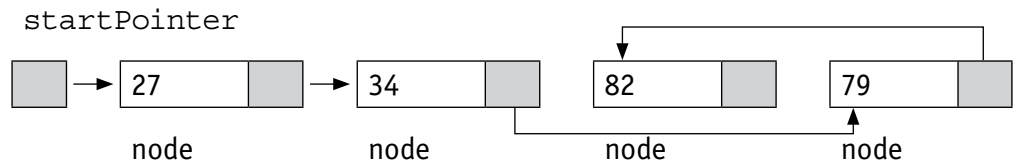
▲ Figure 10.12 Linked list
