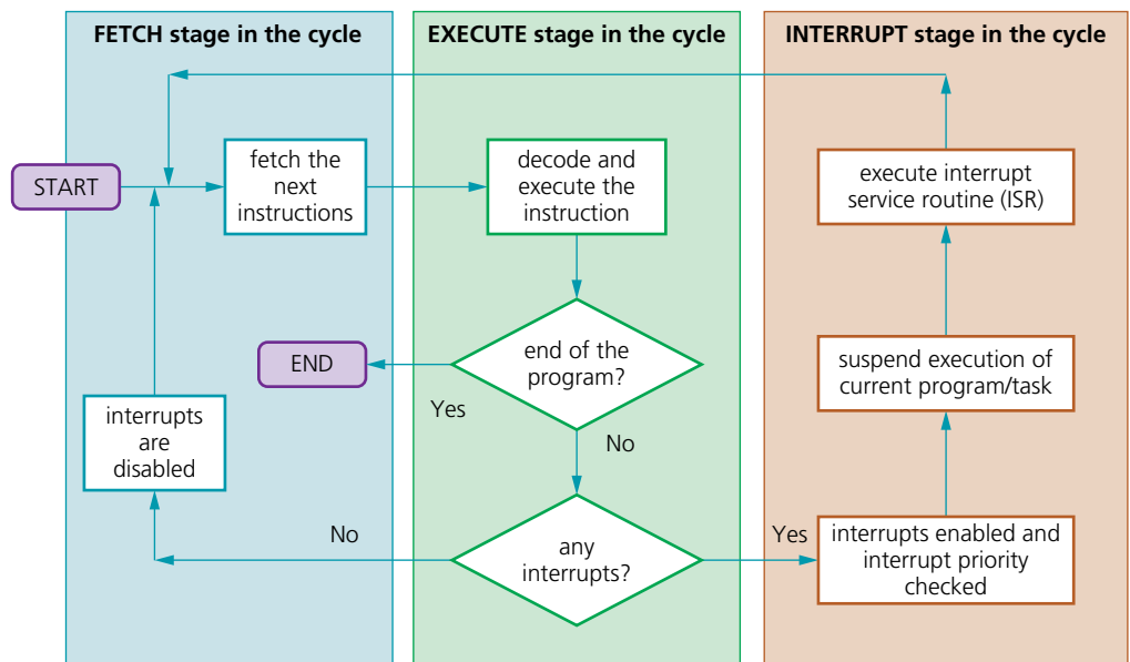
▲ Figure 4.6 The interrupt process during the fetch-execute cycle
