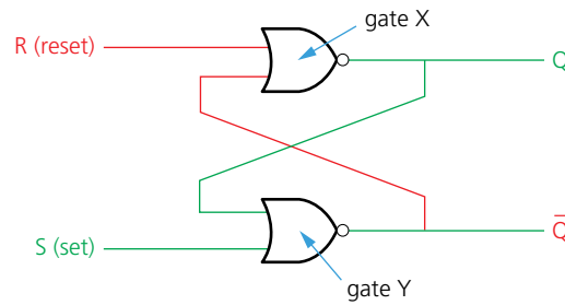
▲ Figure 15.15 SR flip-flop circuit
