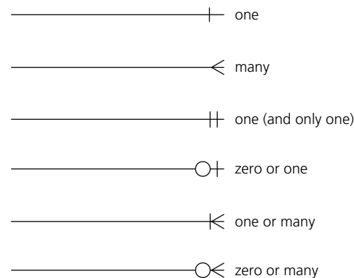
▲ Figure 8.4 Cardinality of relationships
