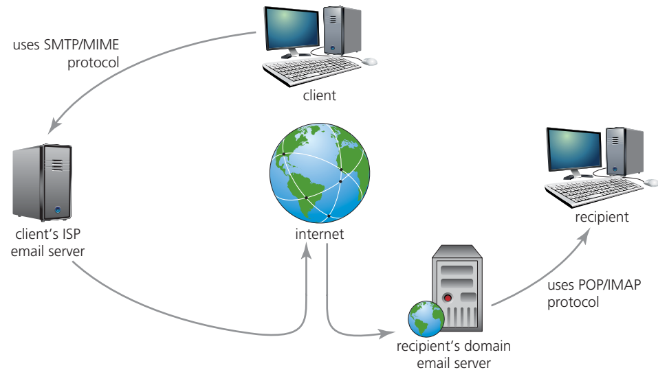
▲ Figure 14.4 Detailed view of email protocol set up
