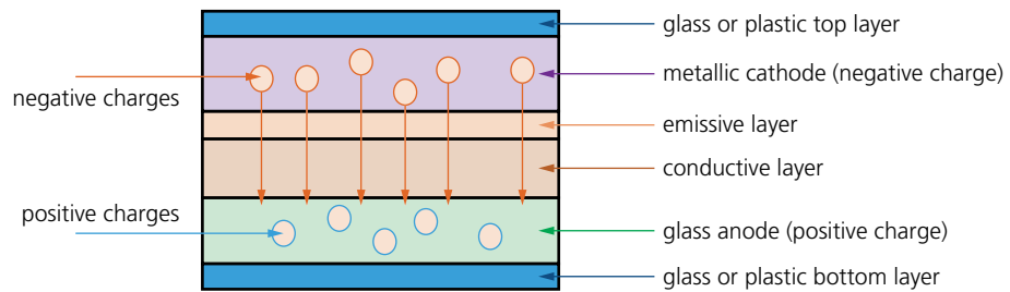
▲ Figure 3.17 Simplified form of how OLED technology works
