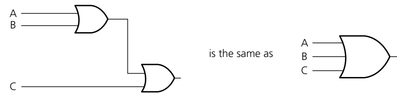
▲ Figure 3.34 Multi-input OR gate
