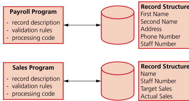
▲ Figure 8.1 File-based approach
