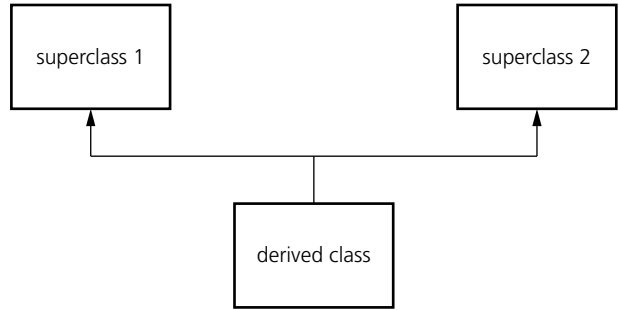
▲ Figure 20.3 Inheritance diagram – multiple inheritance
