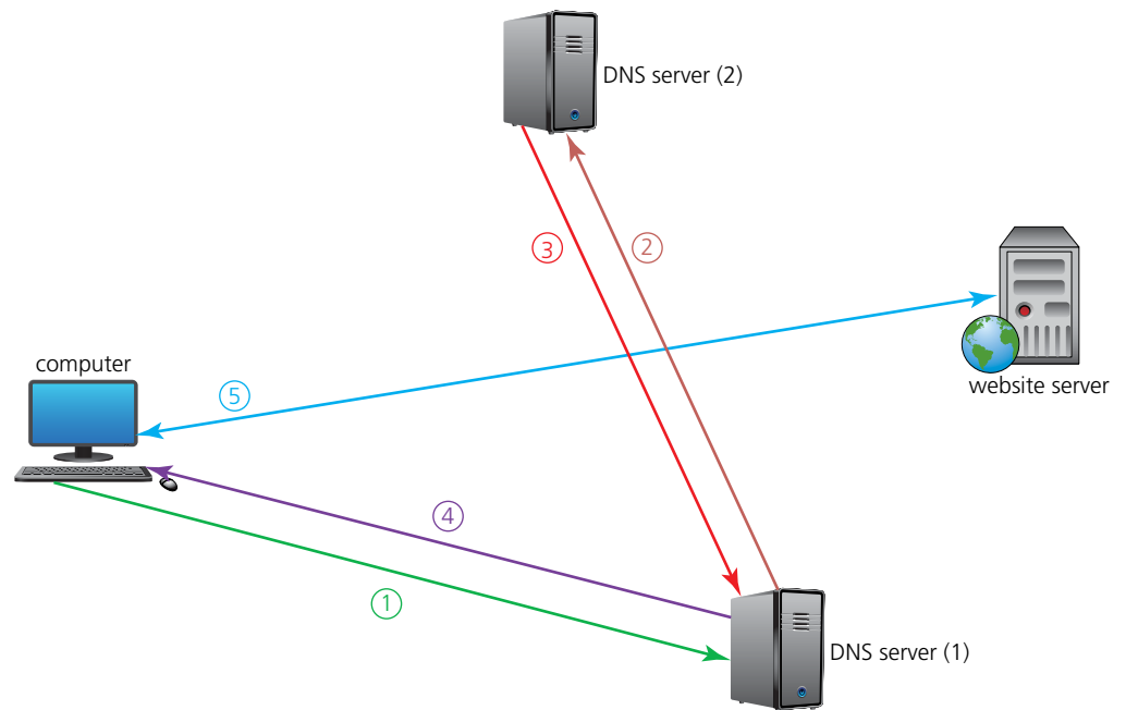
▲ Figure 2.25 An example of the DNS process
